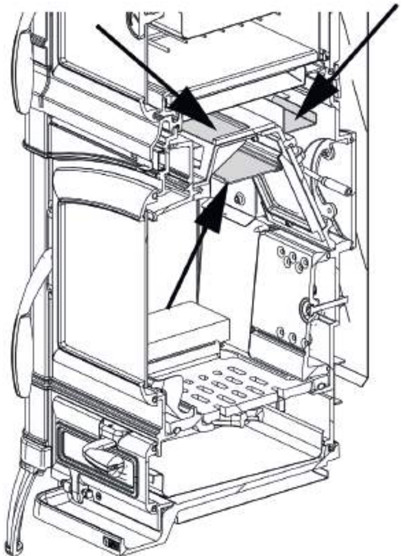
2 - SMOKE BAFFLE
